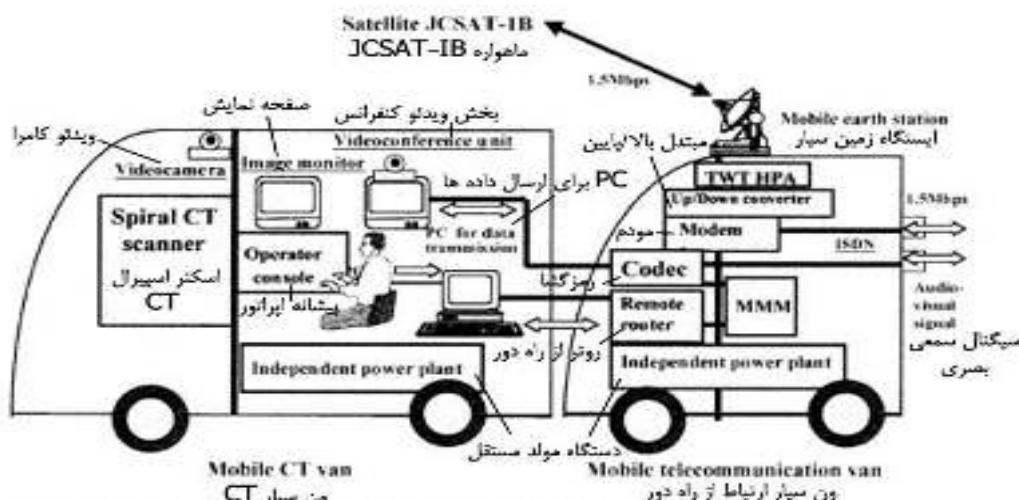
Fig. 1. Schematic diagram of the mobile unit housing spiral CT and telecommunication equipment.
